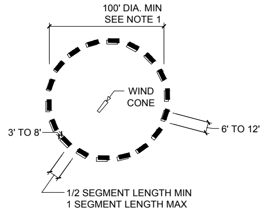
Typical 10' Model Layout
