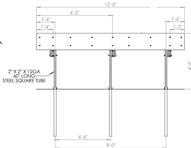
Hali-Brite® Model HB-5340-12-3
