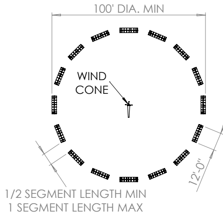
Typical 12' Model Layout
