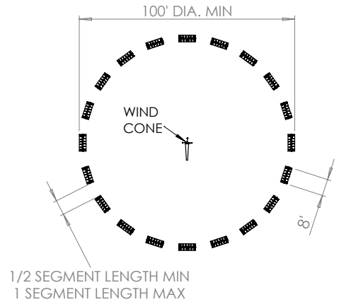
Typical 8' Model Layout
